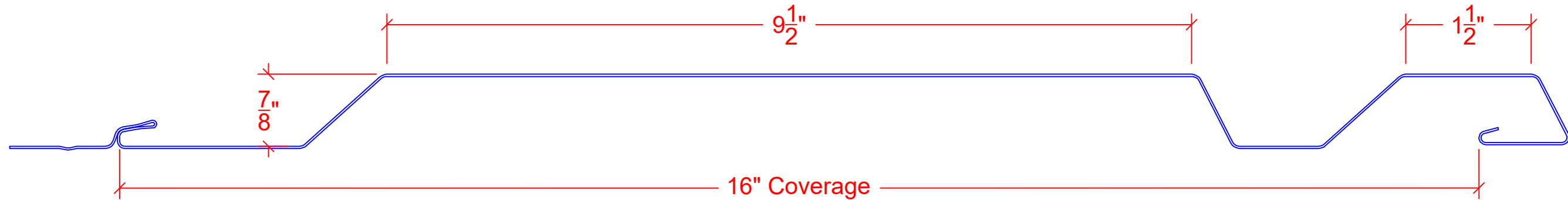
PWP 16-2 Panel
