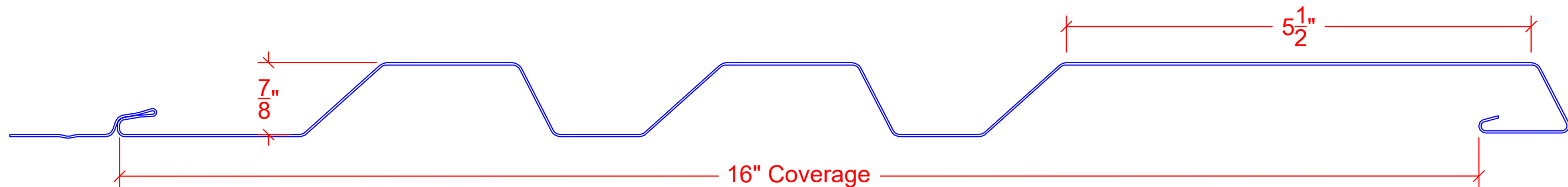
PWP 16-3 Panel
